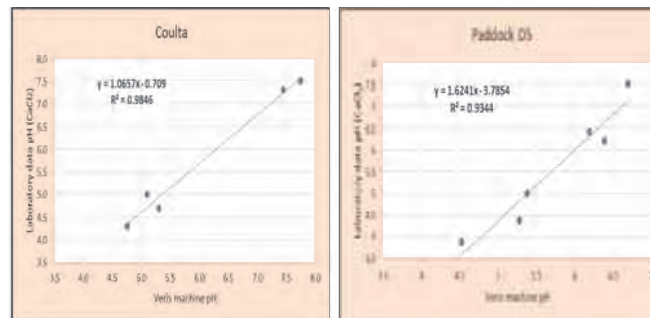
Figures 3a and b: Show examples of calibration between machine pH and laboratory pH data (1:5 CaCl 2 ). The difference between the two calibration lines emphasises the need for a calibration curve to be produced for every paddock.
